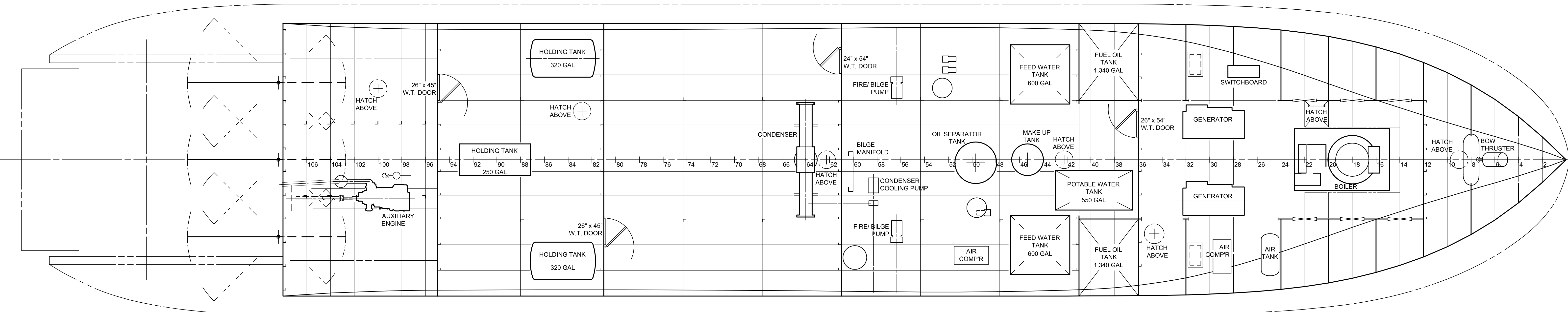
HULL PLAN
