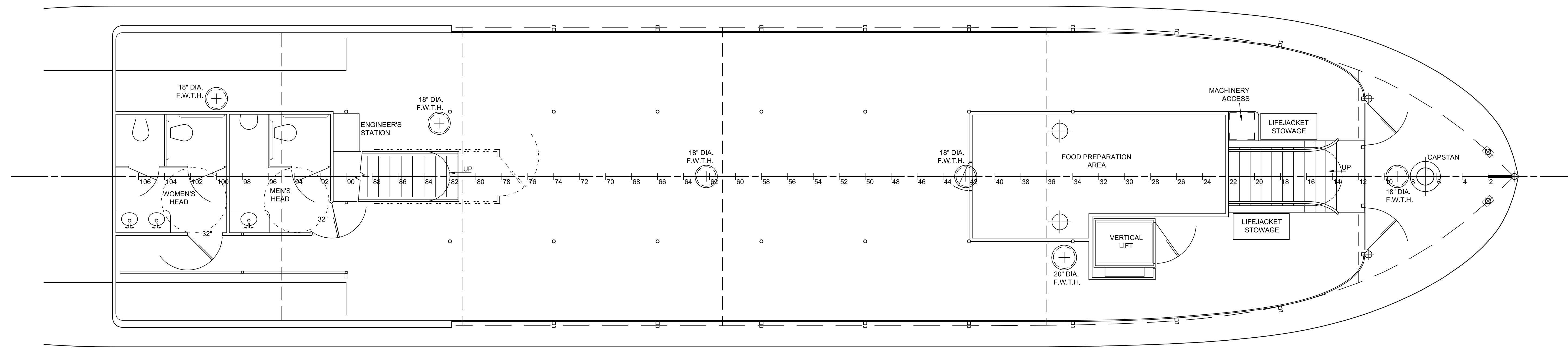
MAIN DECK PLAN
