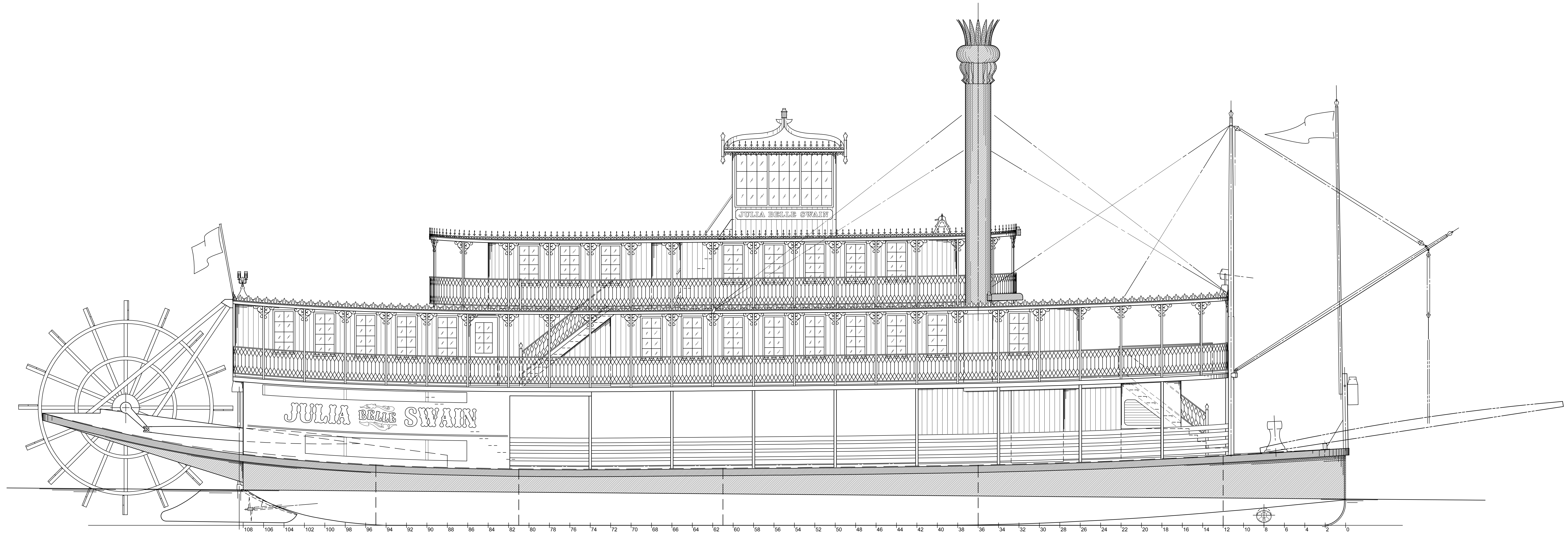
STARBOARD PROFILE
