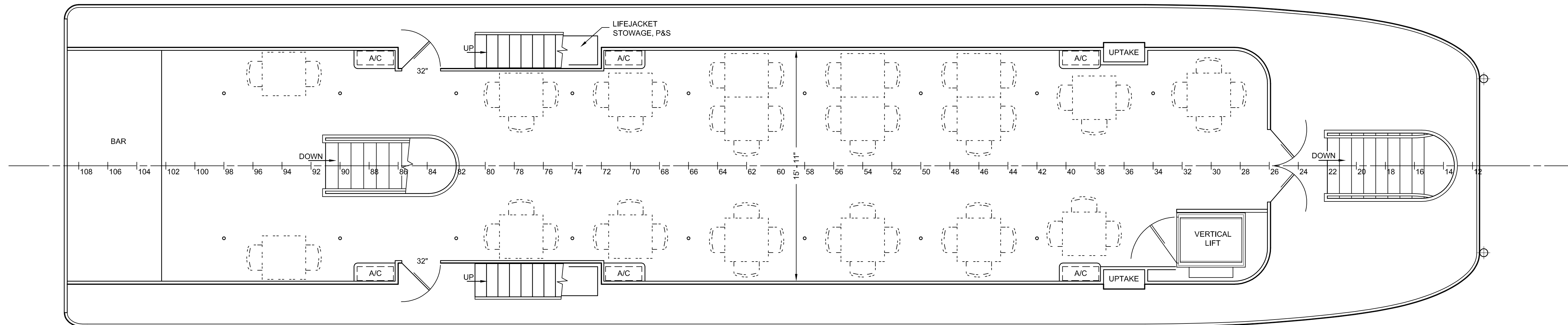
BOILER (01) DECK PLAN
