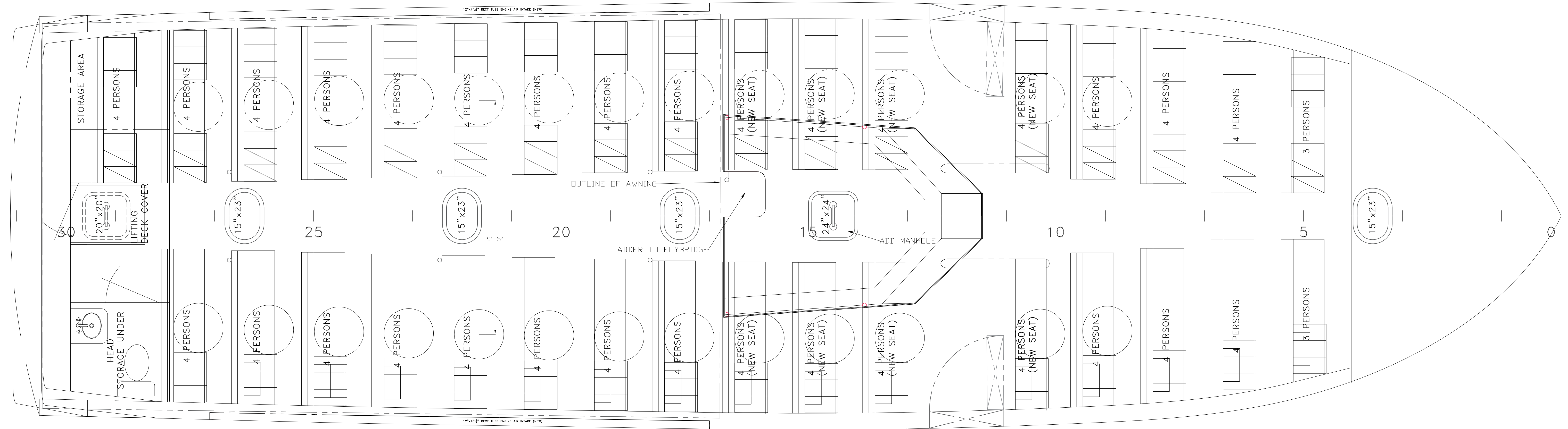
MAIN DECK ARRANGEMENTS
