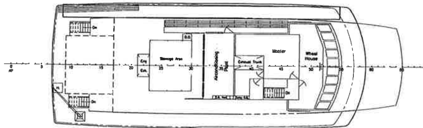
BRIDGE DECK
