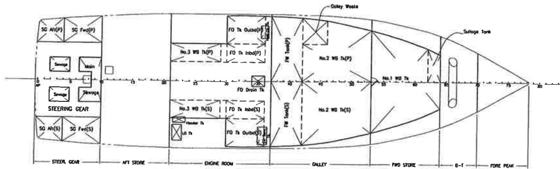
HOLD PLAN
