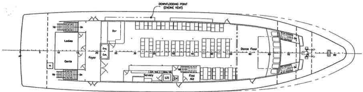
UPPER DECK
