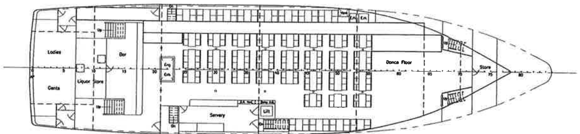
MAIN DECK
