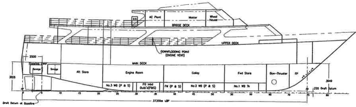
INBOARD PROFILE
