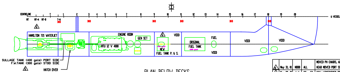
PLAN BELOW DECKS
