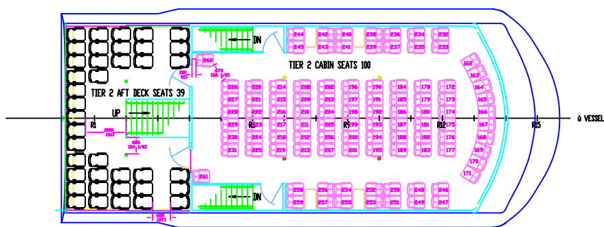
PLAN AT TIER 2 DECK
