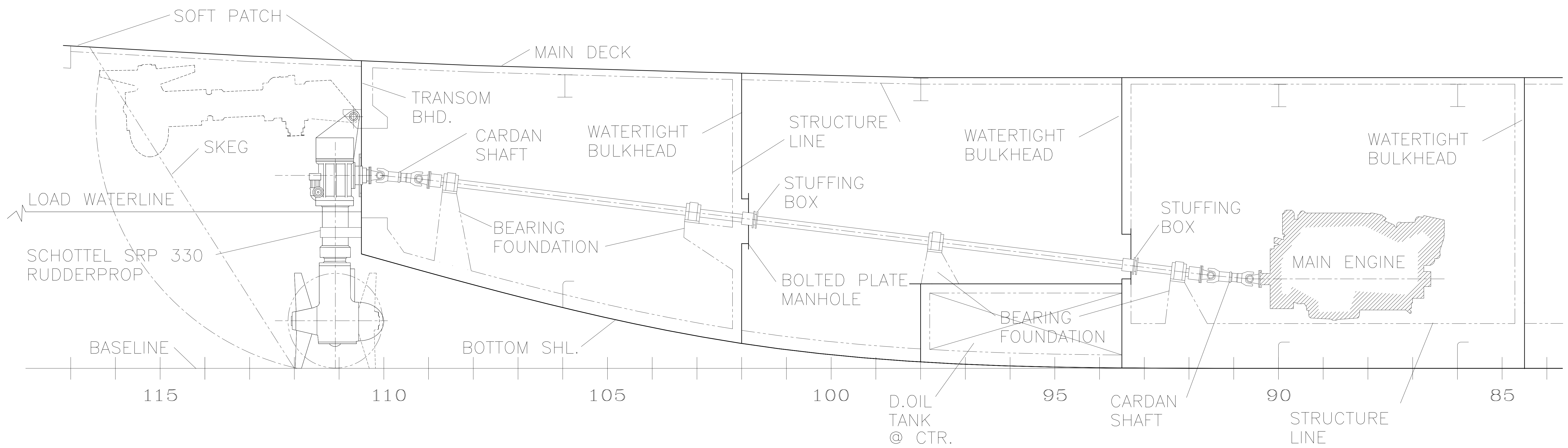
PROFILE : Z-DRIVE ARRANGEMENT
