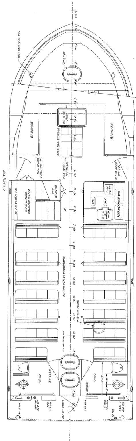
MAIN DECK PLAN
