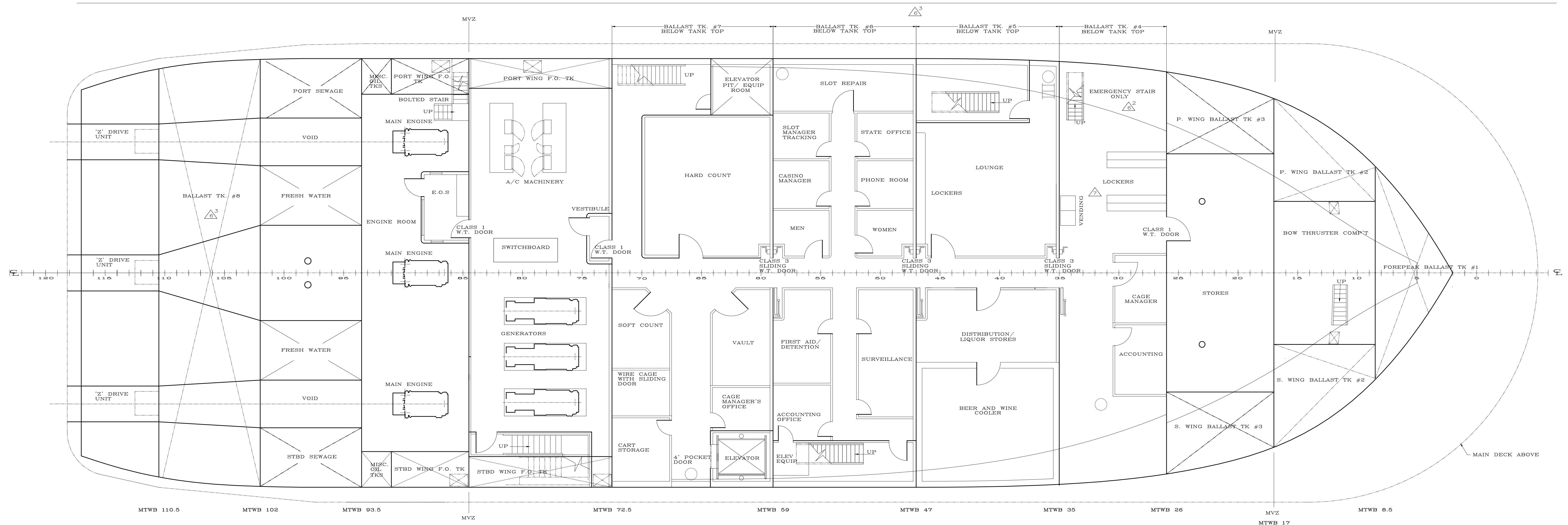
LOWER DECK
