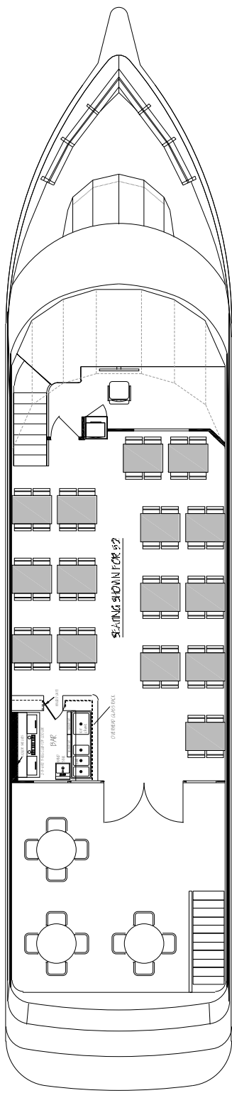
UPPER DECK ARRANGEMENT
