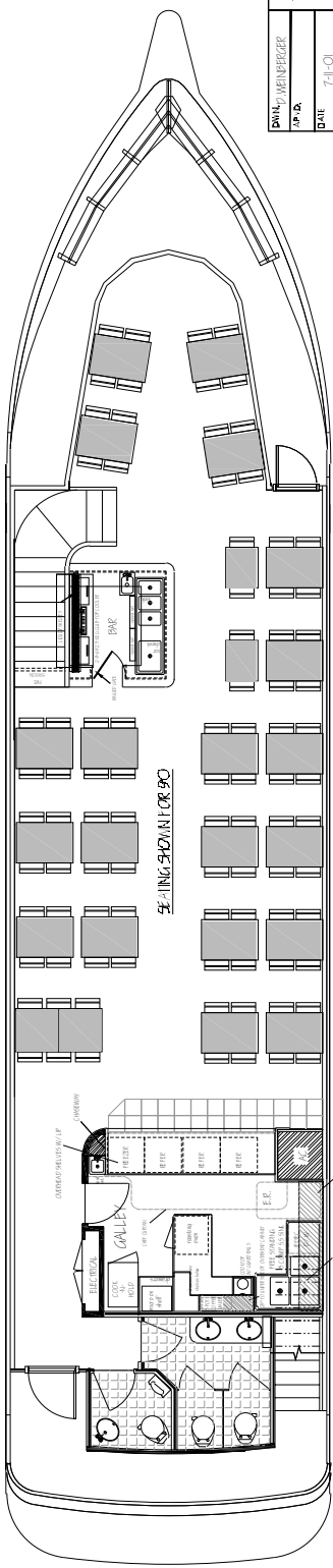
MAIN DECK ARRANGEMENT
